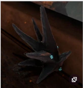
Vitrific Outcrop
